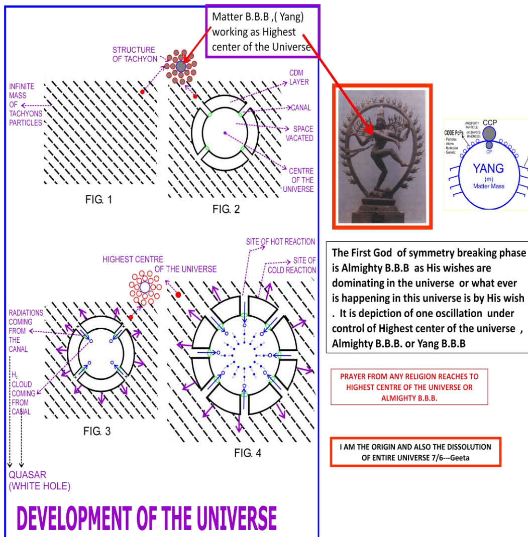
Figure 9.1 Hoyle Narlikar Universe OR Universe "I"
