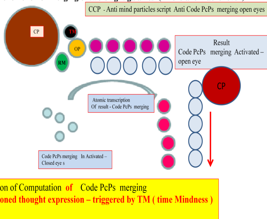
Fig 17 Phenomenon of computation of thought expression of phenomenon of merging ( micro level )
