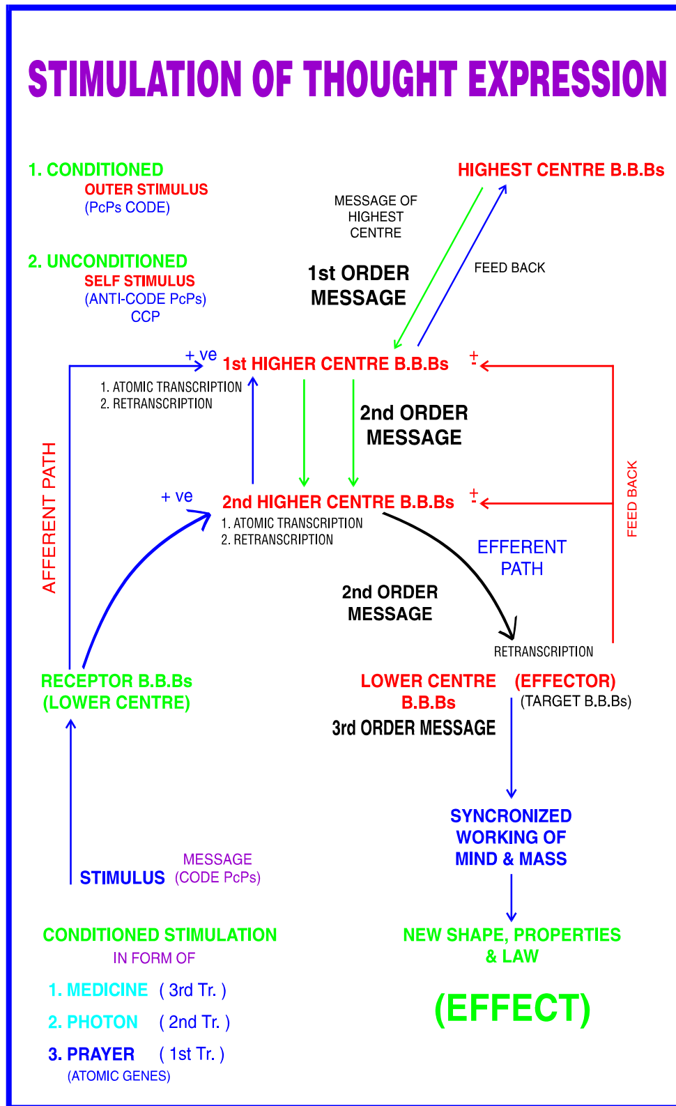
Fig. 7 Conditioned and Unconditioned thought expressions
