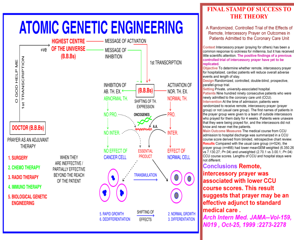
Fig . 4.1 A.G.E and Final stamp of success to New Theory[6]
