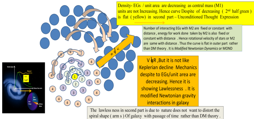
Fig 21 .1 The lawless ness in second part is due to nature does not want to distort the spiral shape ( arm s) Of galaxy rapidly with passage of time , hence number of interacting EGs with M2 are fixed or constant with distance , energy for work done taken by M2 is also fixed or constant . Hence rotational velocity of stars or M2 are same with distance . Thus the curve is flat in outer part . rather than DM theory . It is Divine Modified Newtonian Dynamics or Divine MOND
