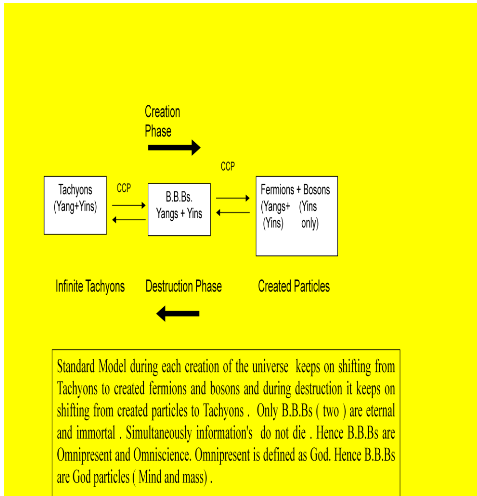
Fig .3.1 one creation and destruction cycle [4]
