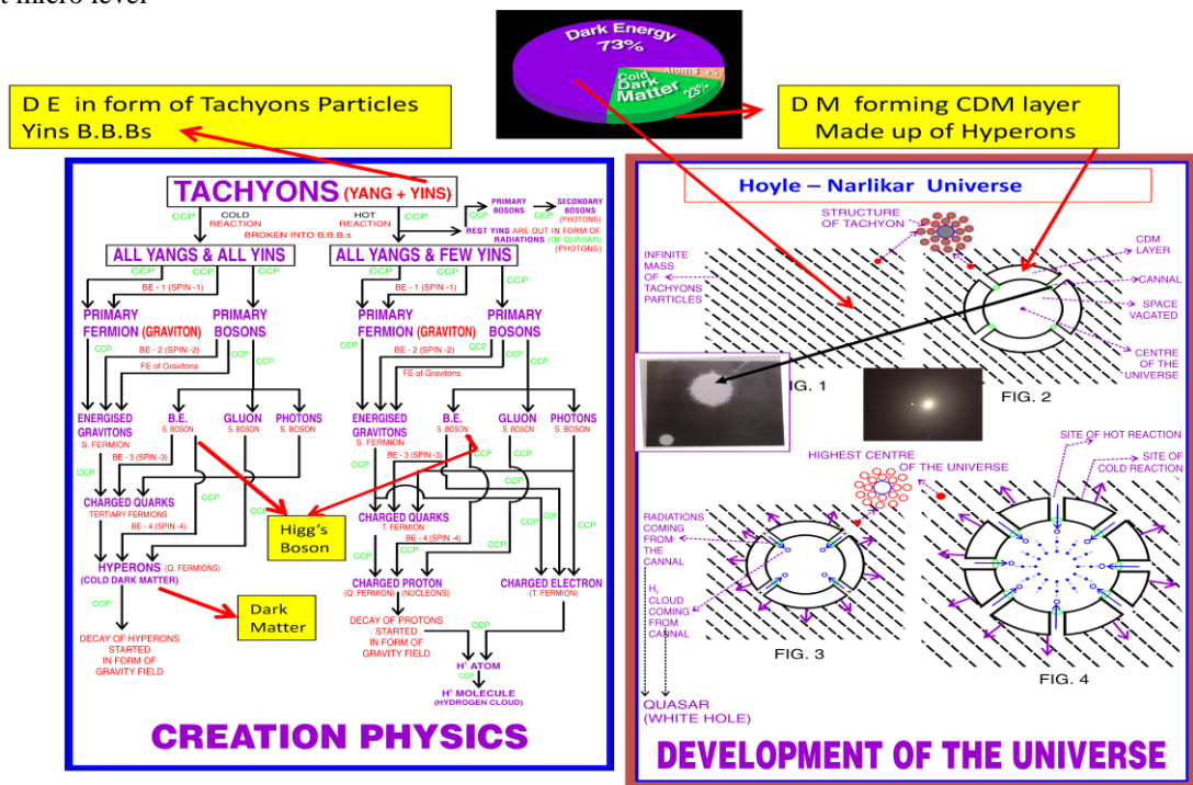
Fig 11 structural configuration of DM and DE at macro level [9]
