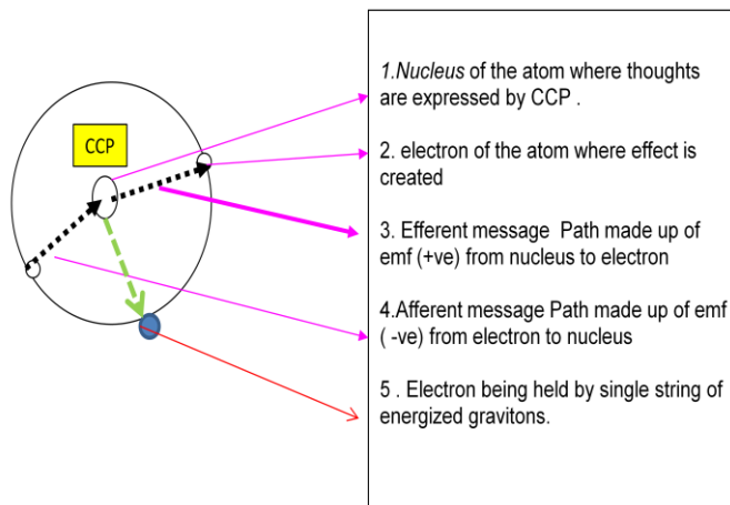
Fig 14 working of hydrogen atom – Divine MONB Theory
