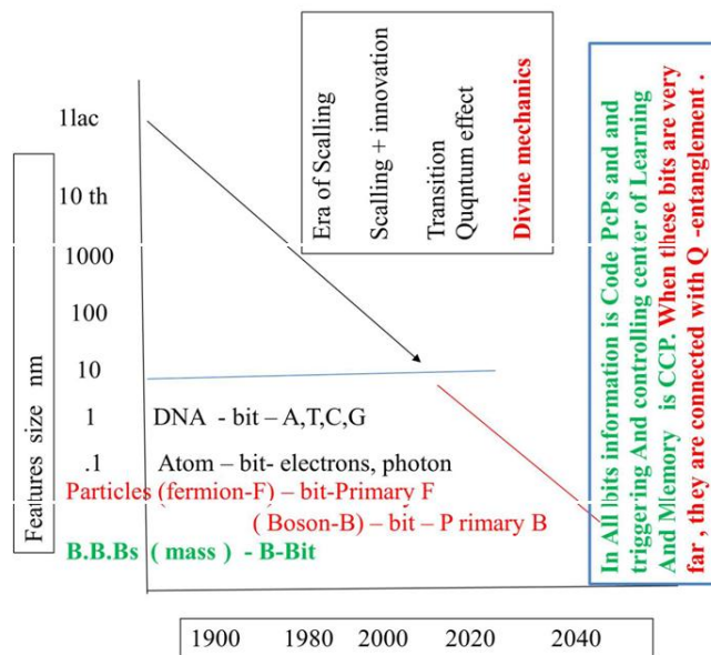
Fig 13- The Theory of Computers and Brain are same – DIVINE MECHANICS ( Structural and Functional smallest Bit ( mass ) is B-Bit of the universe and the Divine Mechanical Unit is CCP , Code PcPs and CP.)
