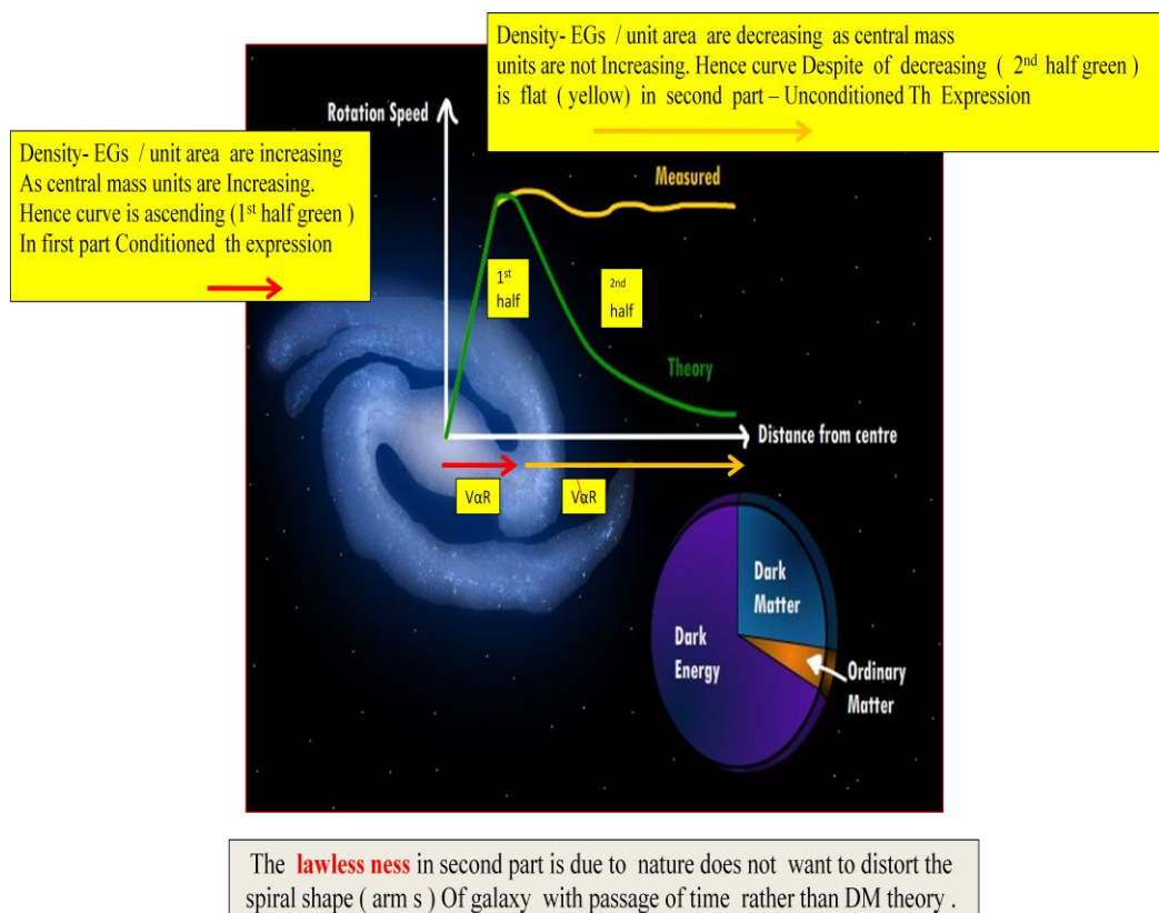
Fig 21 .2 Inner curve ( first part –green ) is designed by conditioned thought stimulation and the outer curve ( second part - yellow ) is designed by unconditioned thought expression of CCP or Divine Modified Newtonian Dynamics (Divine MOND)
