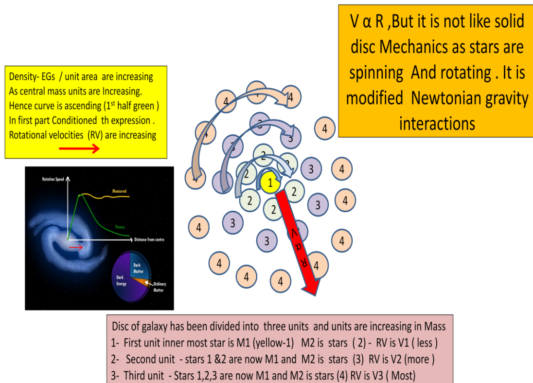
Fig 20 V \propto R ,But it is not like solid disc Mechanics as stars are spinning And rotating . It is modified Newtonian gravity interactions or Modified Newtonian Dynamics which are trigged by mind
