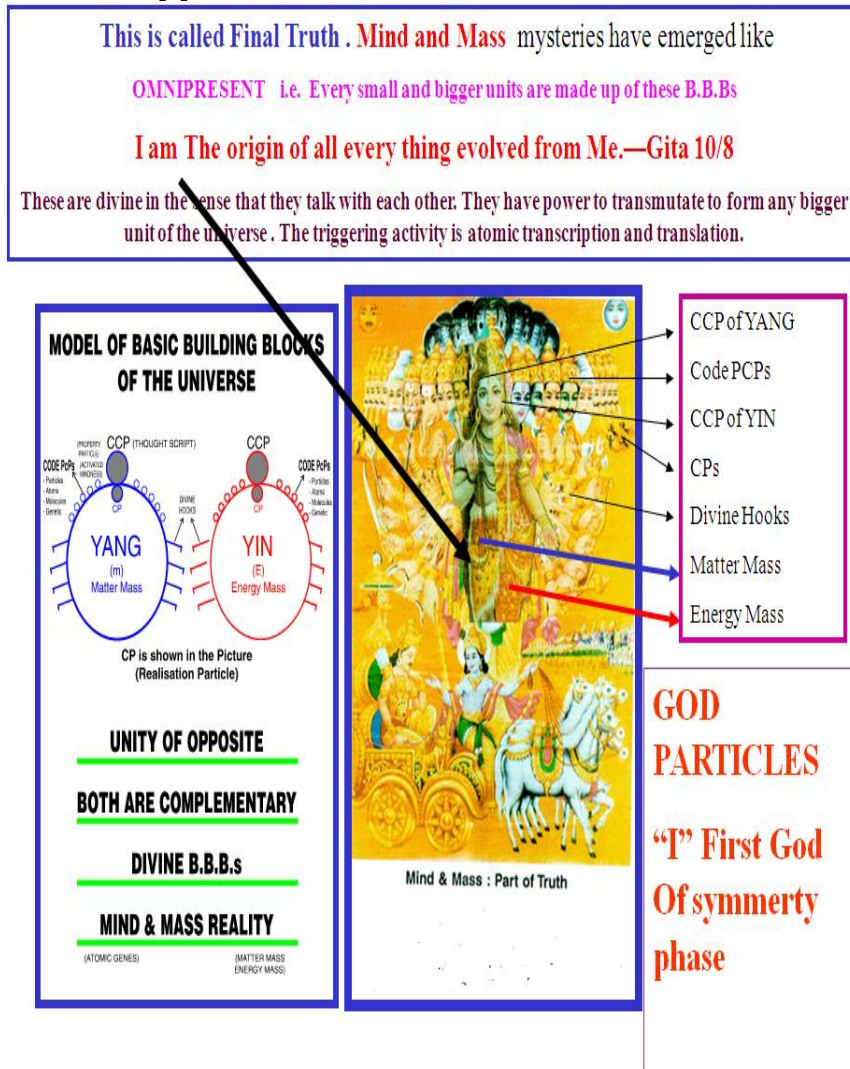
Fig. 1 Divine Mechanics Unit – CCP, CP and information s – Code PcPs with B-Bit – Mass
