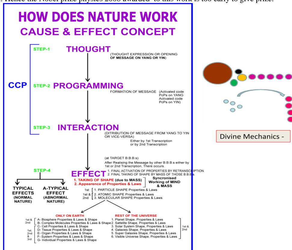
Fig. 6 Divine Mechanics – How Does Nature work ?
